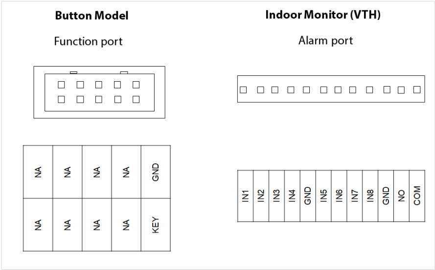
Figure 1-12 Cable connection
